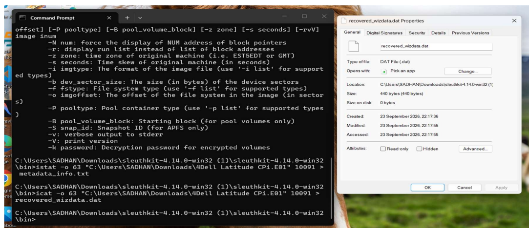
Figure 6: Successful extraction and recovery of wizdata.dat using the icat command
