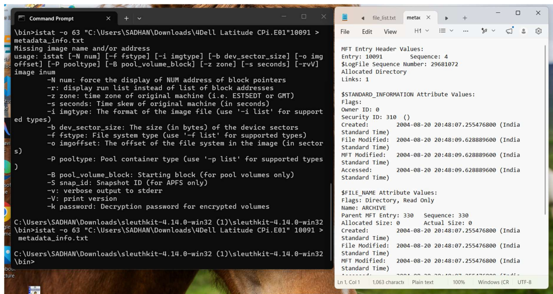
Figure 5: Viewing detailed file metadata (istat output) for inode 10091
