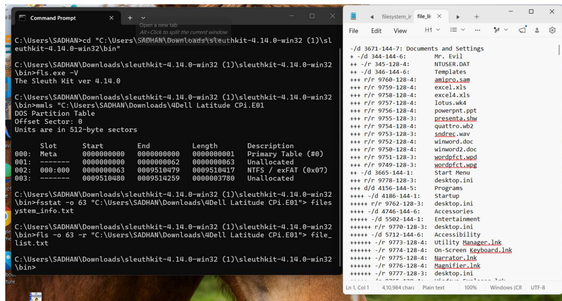
Figure 4: Searching file_list.txt to identify the deleted wizdata.dat file at inode 10091
